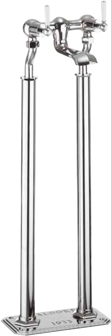
Bath filler WF322DC_LV £505.00 Deck mounted Water pressure: HP1 A: 246mm B: 194mm
