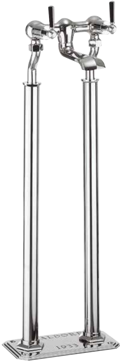
Bath filler WF322DC_BLV £505.00 Deck mounted Water pressure: HP1 A: 246mm B: 194mm
